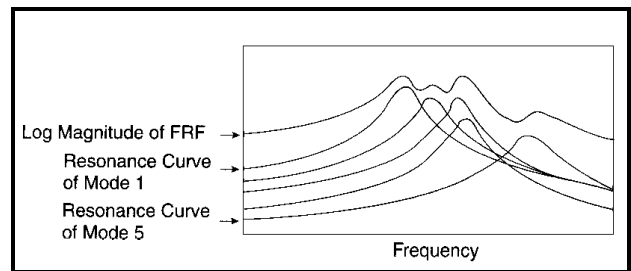
Figure 6. FRF as Sum of Resoance Curves.
