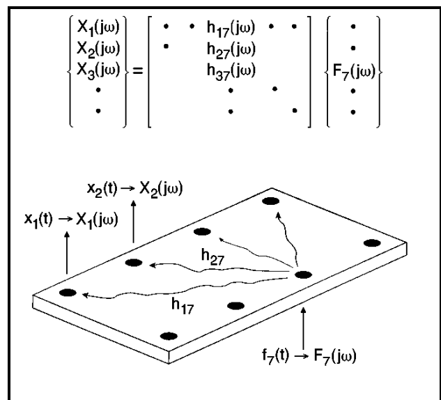
Figure 2. FRF Measurements on a Structure.
