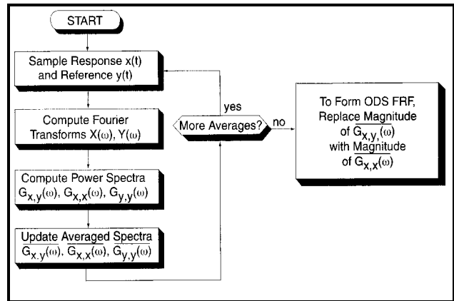
Figure 9. Tri spectrum Averaging to Compute ODS FRF
