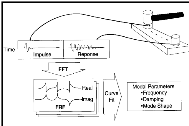
Figure 3. Impact Testing
