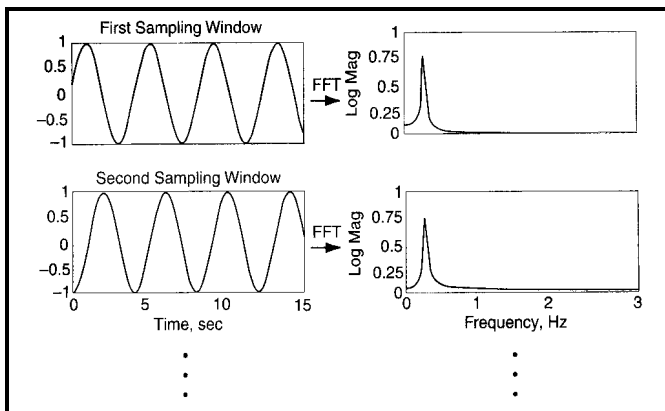
Figure 8. Steady State Operation.
