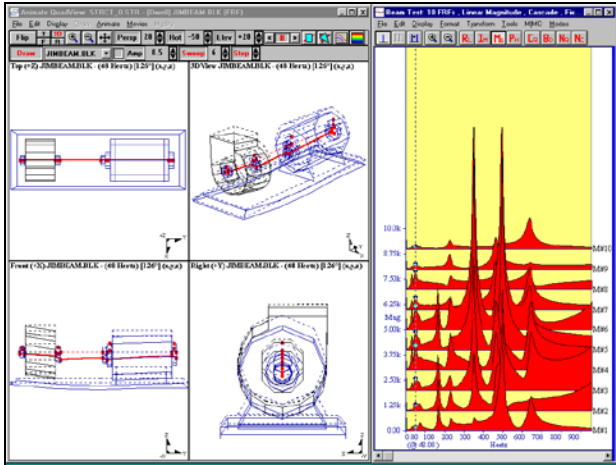
Figure 10. Animation of ODS FRF Data.
