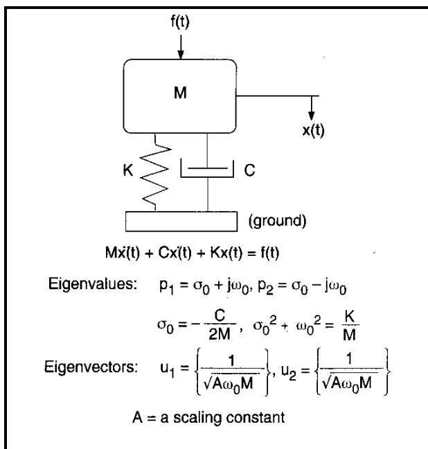
Figure 5. Mass/Spring/Damper SDOF Vibrator
