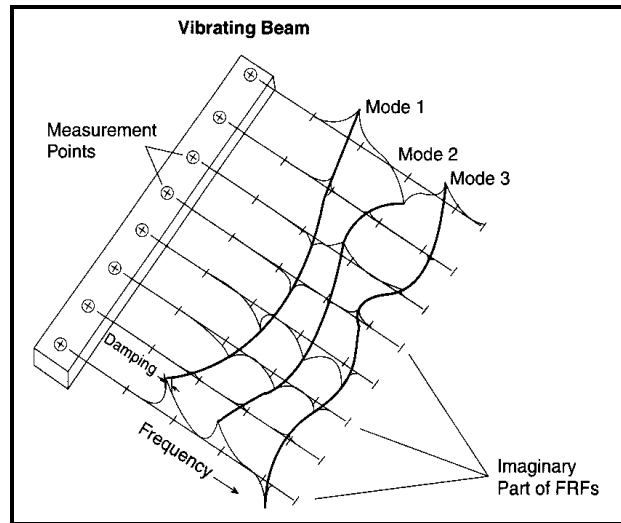
Figure 4. Curve Fitting FRF Measurements.
