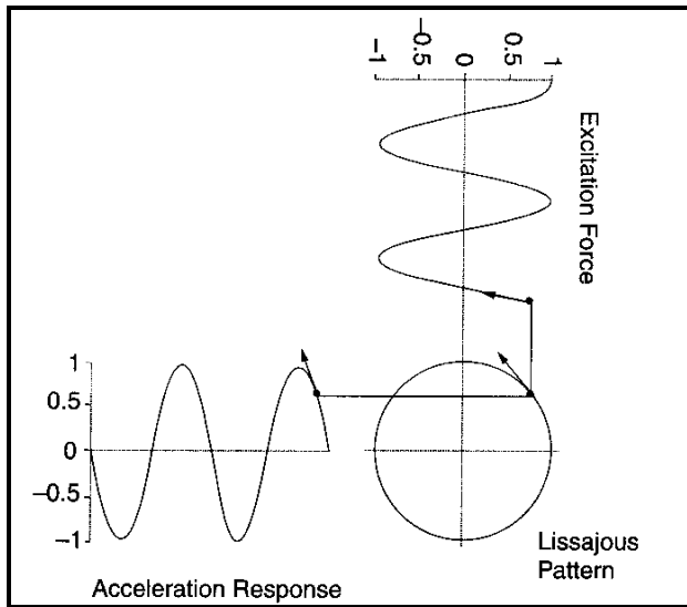
Figure 1. Lissajous Pattern Indicating a Pure Mode.
