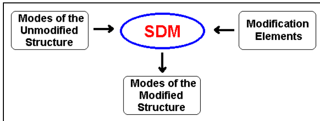
Figure 4. SDM Procedure.
