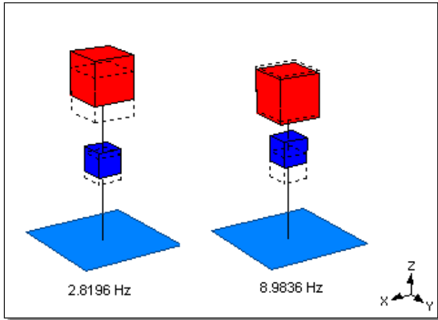
Figure 6. Modes of the 2 DOF Structure.
