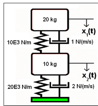
Figure 5. 2-DOF Structure.
