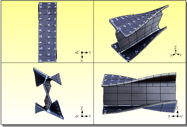
Figure 9E. 1805 Hz FEA Mode Shape.
