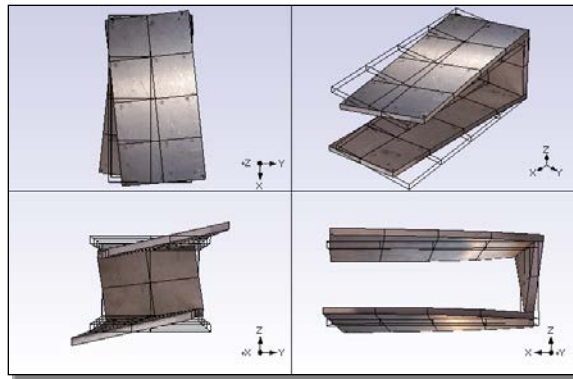
Figure 5A. 150 Hz FEA Mode Shape.
