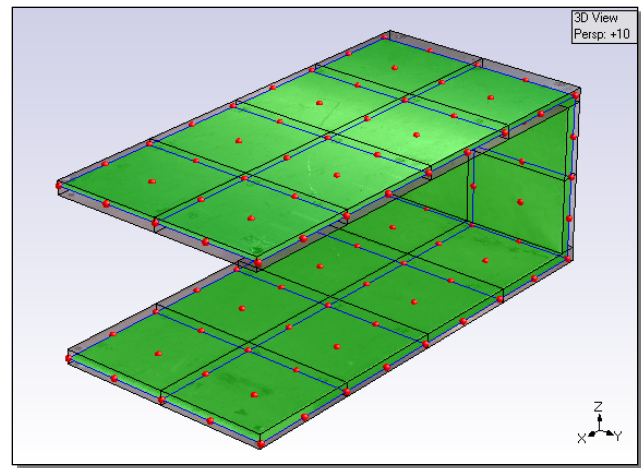
Figure 3. Extruded Cross Section of the Photo Model.
