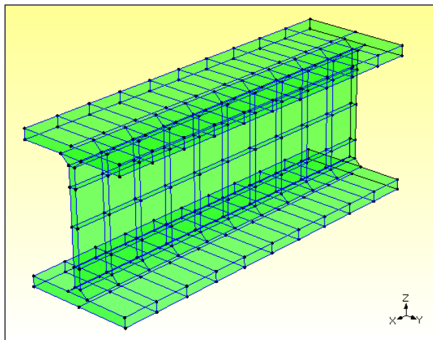
Figure 8. I Beam Extruded from a Cross Section of the Photo Model.
