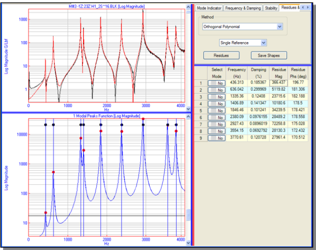
Figure 10. FRF Curve Fit to Extract EMA Modes.
