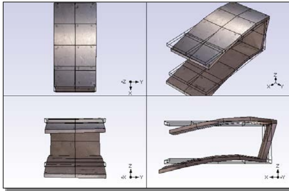
Figure 5B. 216 Hz FEA Mode Shape.
