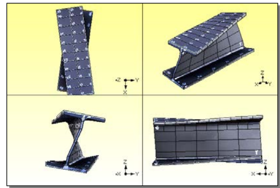
Figure 9A. 461 Hz FEA Mode Shape.
