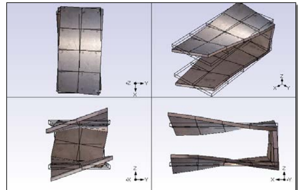
Figure 5E. 451 Hz FEA Mode Shape.
