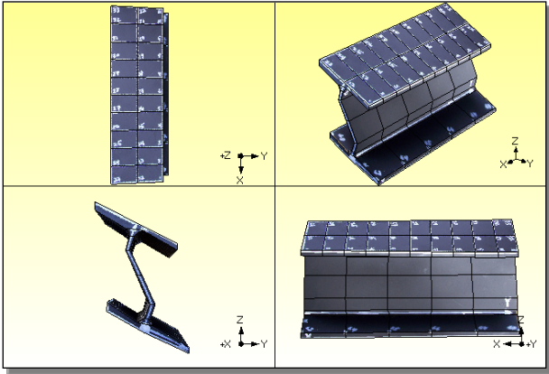
Figure 9D. 1399 Hz FEA Mode Shape.
