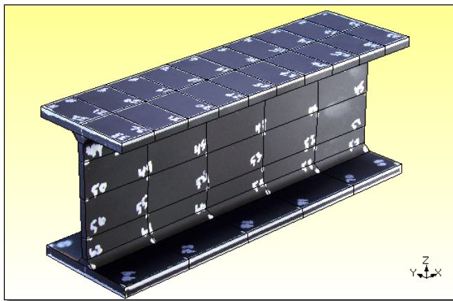
Figure 6. Photo Model of the I Beam.
