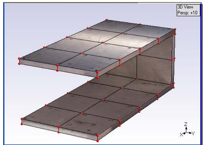
Figure 1. Photo Model of the 3-Plate Beam.
