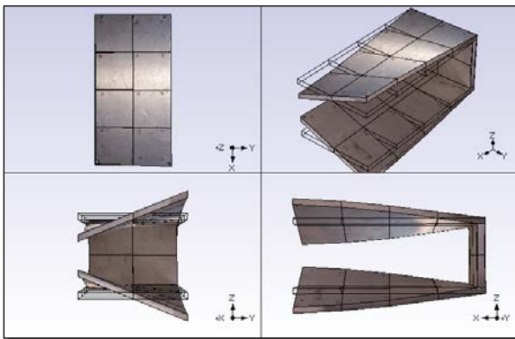
Figure 5C. 311 Hz FEA Mode Shape.
