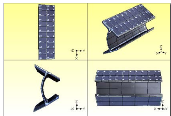
Figure 9B. 574 Hz FEA Mode Shape.
