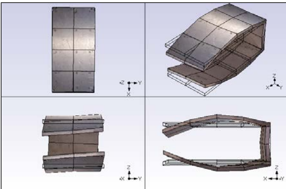
Figure 5D. 428 Hz FEA Mode Shape.
