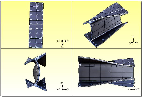
Figure 9C. 1293 Hz FEA Mode Shape.
